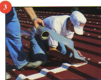
Treating the horizontal seams with Butyl tape
